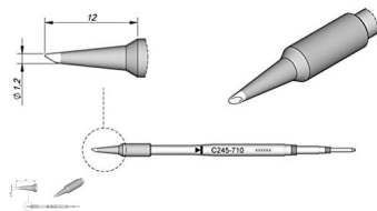
JBC Ponta de solda 1.2mm C245710
